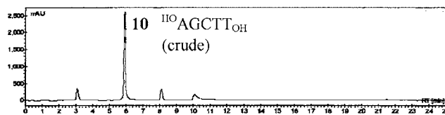
Figure 2. HPLC trace (254 nm) of the crude, fully deprotected pentameric DNA fragment 10 ( \text{HOAGCTT}_{\text{OH}} ).
