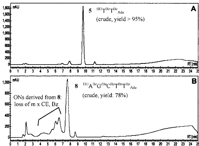
Figure 1. HPLC traces (254 nm) of the crude products after one elongation cycle: (A) \text{HO-T}^{\text{Bz}}\text{T}^{\text{Bz}}\text{Ada} and four elongation cycles (B) \text{HO-A}^{\text{Bz}}\text{G}^{\text{iBu}}\text{C}^{\text{Bz}}\text{T}^{\text{Bz}}\text{T}^{\text{Bz}}\text{Ada} ( 8 ).
